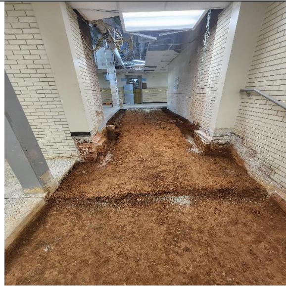
Preparation of subgrade for Ramp
