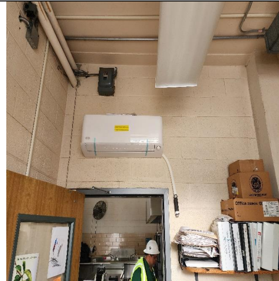
Kitchen Office Unit Install
