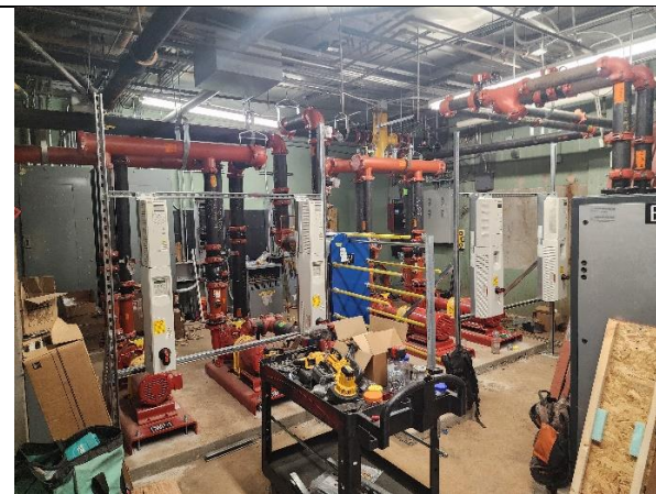
Boiler Room Equipment Install.
